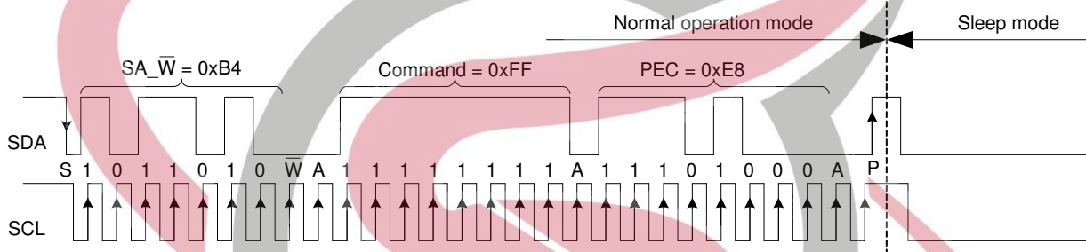
Figure 11: Enter sleep mode command (SA = 0x5A, Command = 0xFF, PEC = 0xE8)
