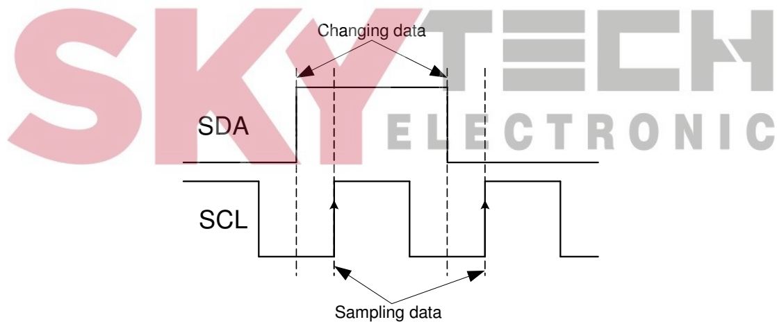
Figure 7: Recommended timing on SMBus
